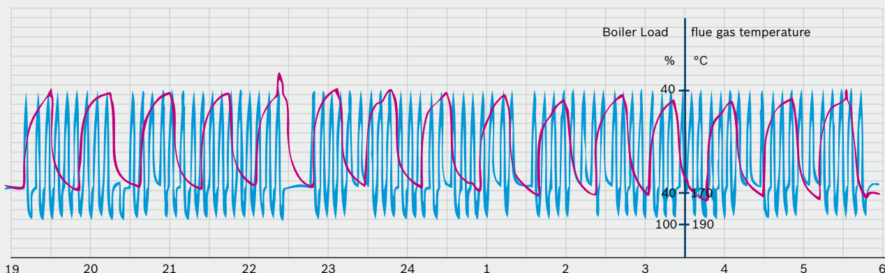
Operational diagrams of gas-fired high-pressure hot water boilers before as well as after correction of its load behaviour in the low-load phase between 7.00 p.m. and 6.00 a.m.
