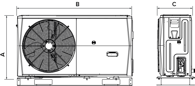
CS2000 AWF 4 R-S a CS2000 AWF 6 R-S
