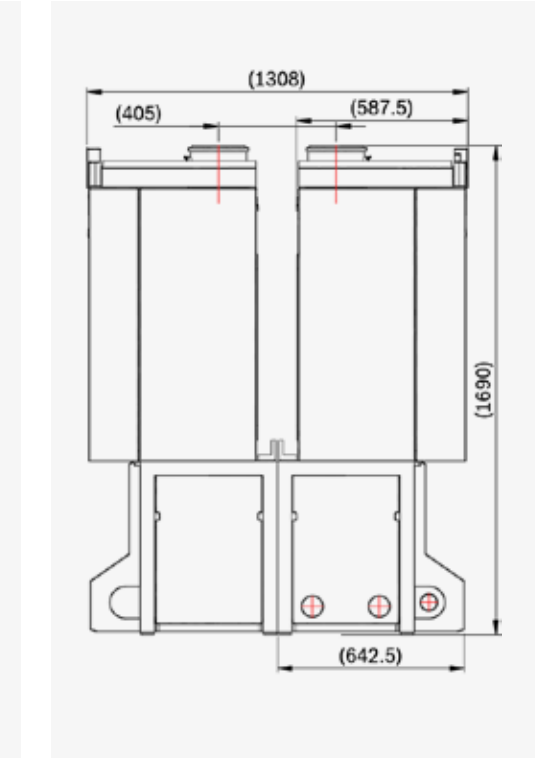
GC7000WP 125 and 145kW
