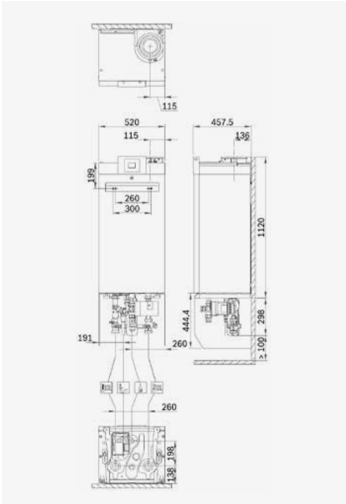
GC7000WP boiler on wall
