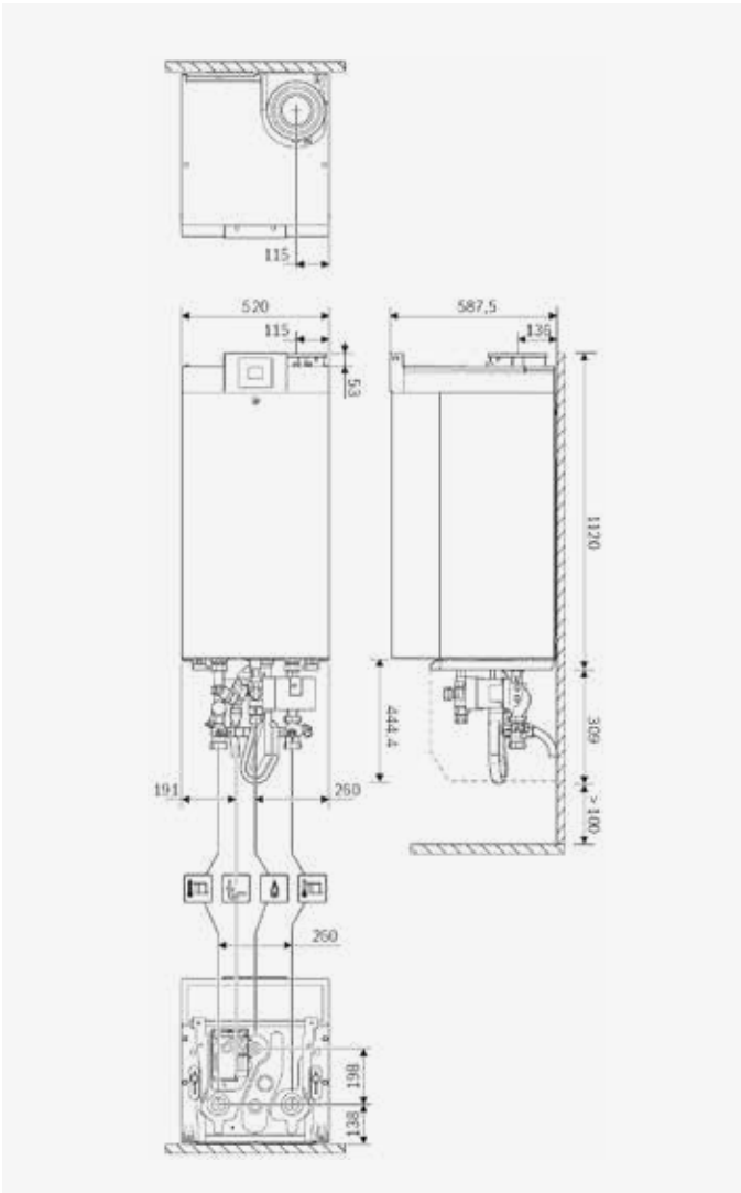
GC7000WP boiler on wall
