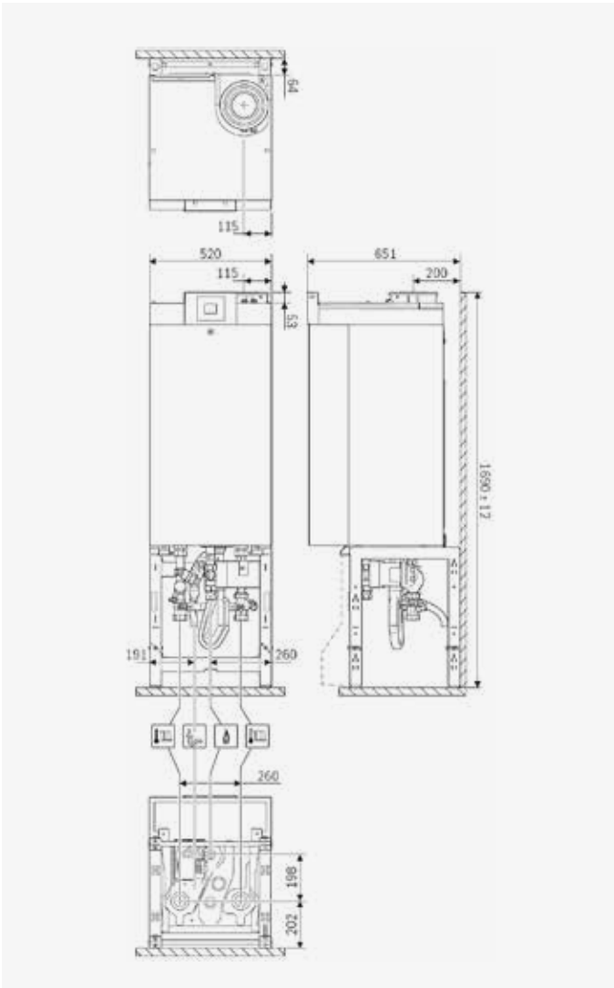
GC7000WP boiler on frame
