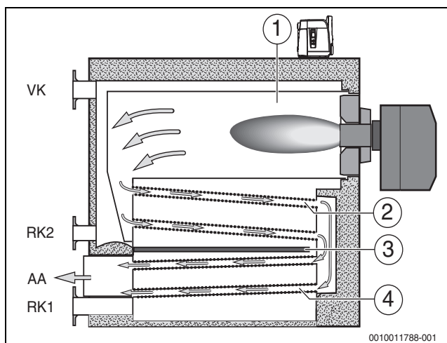
Fig. 1 Function diagram of the path of the products of combustion in the Uni Condens 8000 F 50...115 and Uni Condens 8000 F 145...640 floor standing condensing boilers
