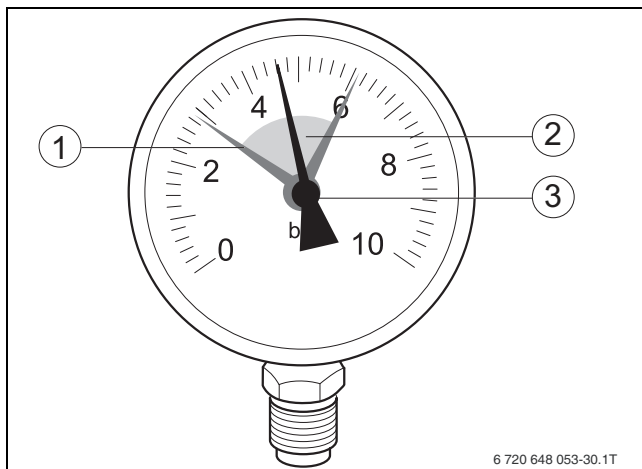
Fig. 3 Pressure gauge for closed heating systems
