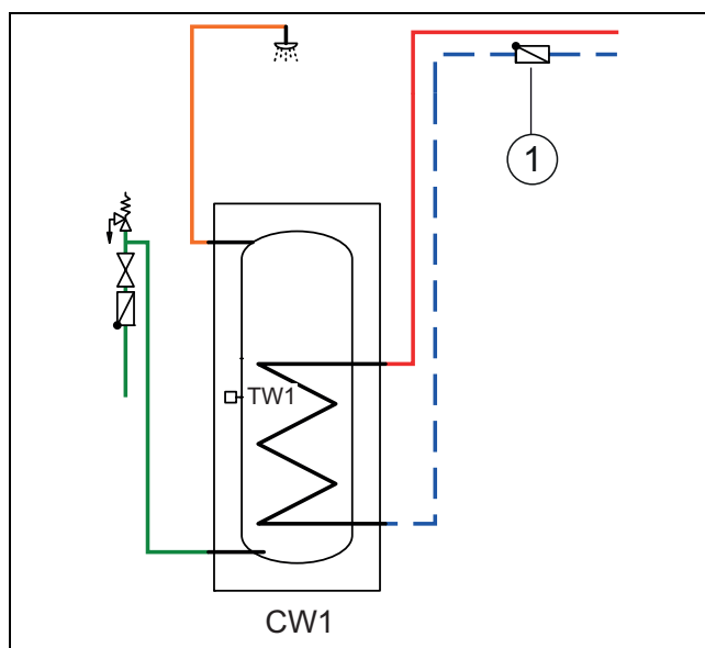
Joon. 24 Boiler
